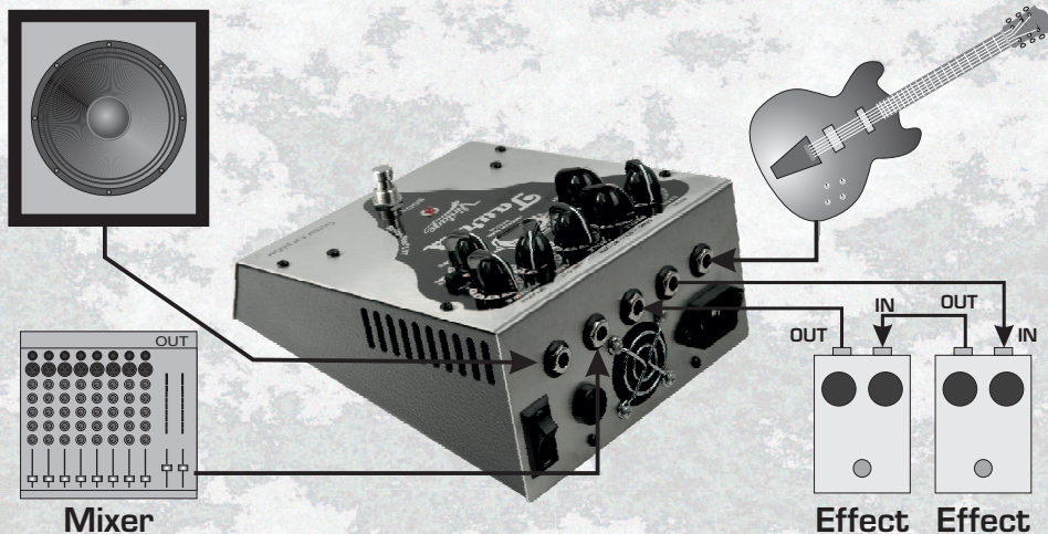
LINE-OUT wire connection
